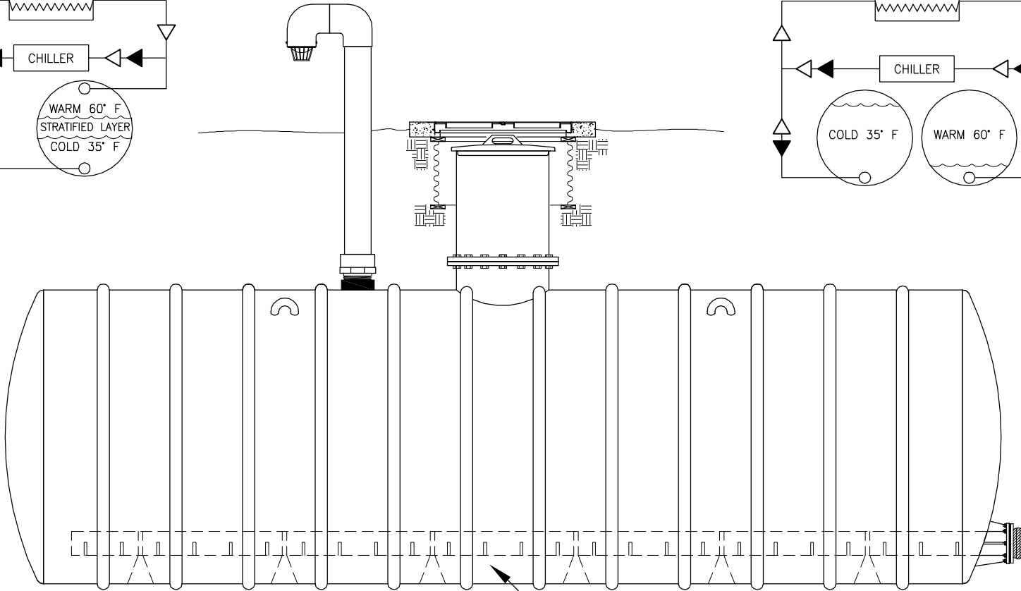
SINGLE TANK SYSTEM
