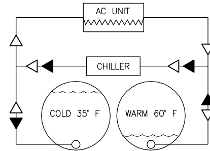
DOUBLE TANK SYSTEM
