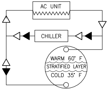
SINGLE TANK SYSTEM
